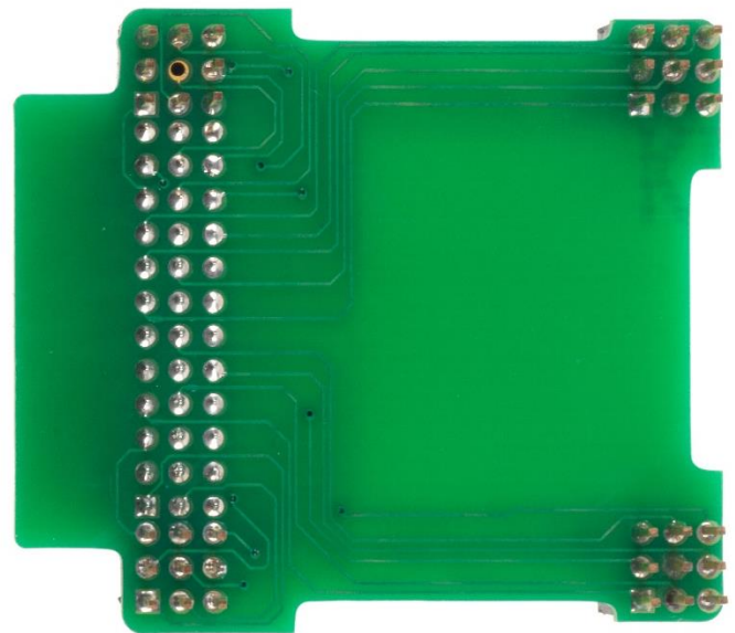
Front and back views of KA1046-01 Side Stack 0 Degree Rotate Components. They snap together without tools.
